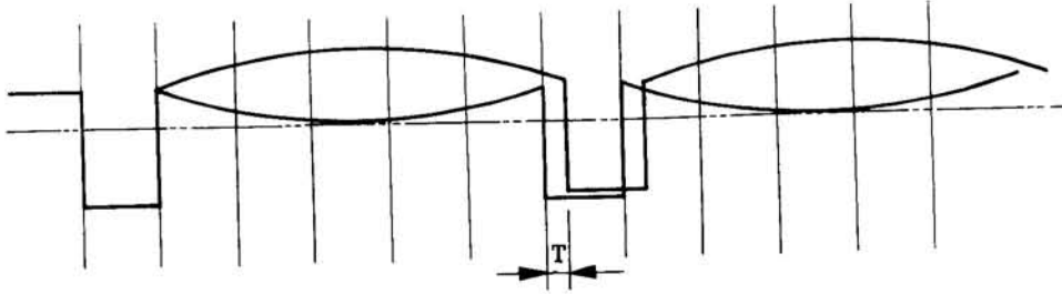
Fig. 9.7 Asymmetry Waveform
