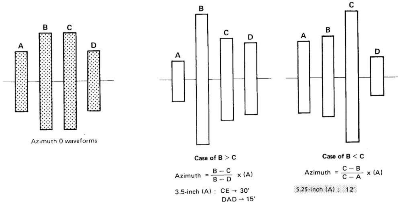
Fig. 9.4 Azimuth Waveforms
